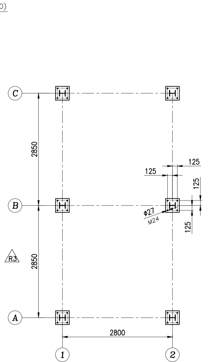
BASE PLATE VIEW
