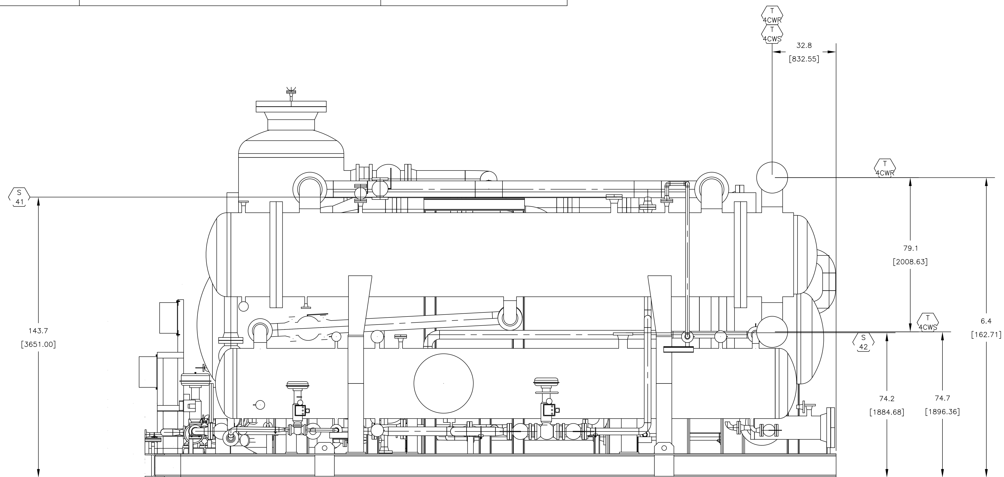
RIGHT VIEW
