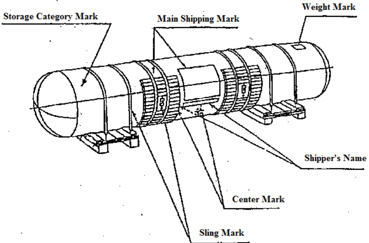
Fig-2: Outside View of SKID, BARE
