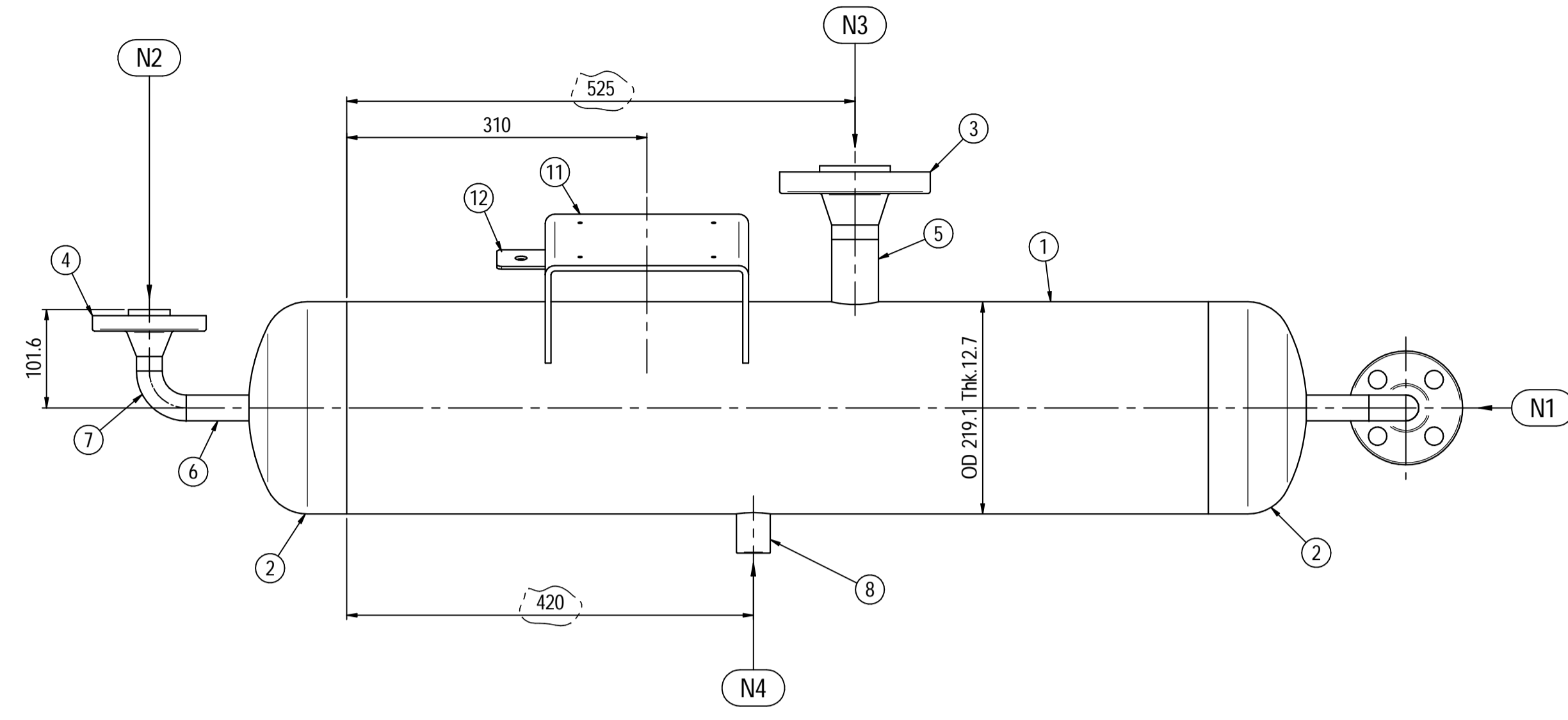
ELEVATION VIEW
